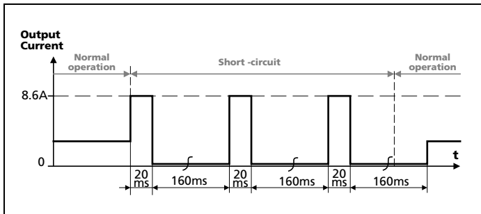
Fig. 6-2 Intermittent current at short circuit, typ.
