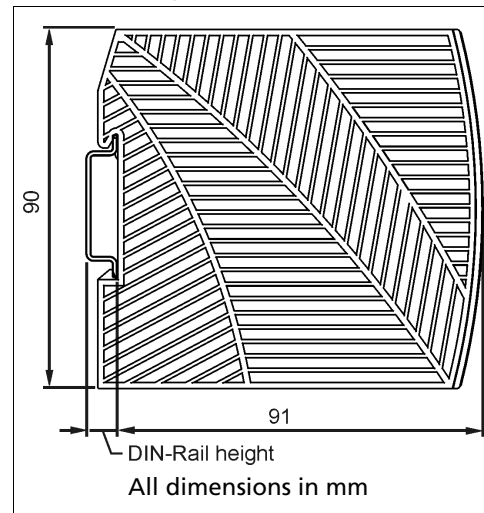
Fig. 20-2 Side view
