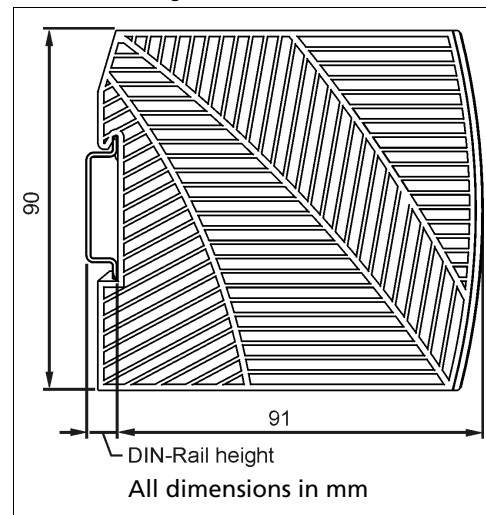
Fig. 20-2 Side view
